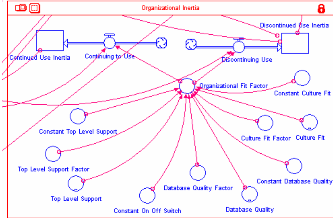
Figure 54: Organizational Inertia Formulated Structure in STELLA
